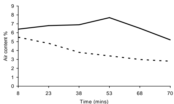
Figure 1 Air content vs mixing time
